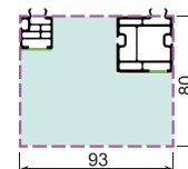
Passive thermal threshold with TOP®
