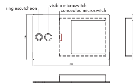
Place of assembly of microswitches.
